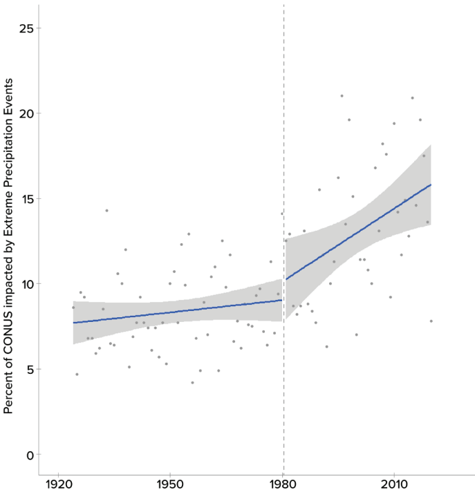
Figure 2: Percent of CONUS impacted by extreme rainfall events, pre- and post-1980. Data source: EPA
