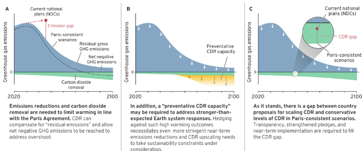
Figure 8. A stylised sketch of the possible scenario pathways that reach net-zero CO 2 and greenhouse gas emissions. Emissions reductions and CO 2 removal (CDR) are needed to limit warming. CDR can compensate for “residual emissions” and allow net-negative GHG emissions to be reached to address overshoot; however, CDR will be limited by land area and other sustainability constraints (Panel A). This implies the need for faster and deeper emissions reductions, reserving CDR to compensate only for residual emissions from “critical needs”. A “preventative CDR capacity” may be required to address unexpected Earth system responses (Panel B). As it stands, there is a gap between country proposals for scaling CDR and conservative levels of CDR in scenarios (Panel C). Reducing the need for preventative CDR capacity will depend on stronger national pledges and implementation of emissions reductions (based on Lamb et al. 2024).
